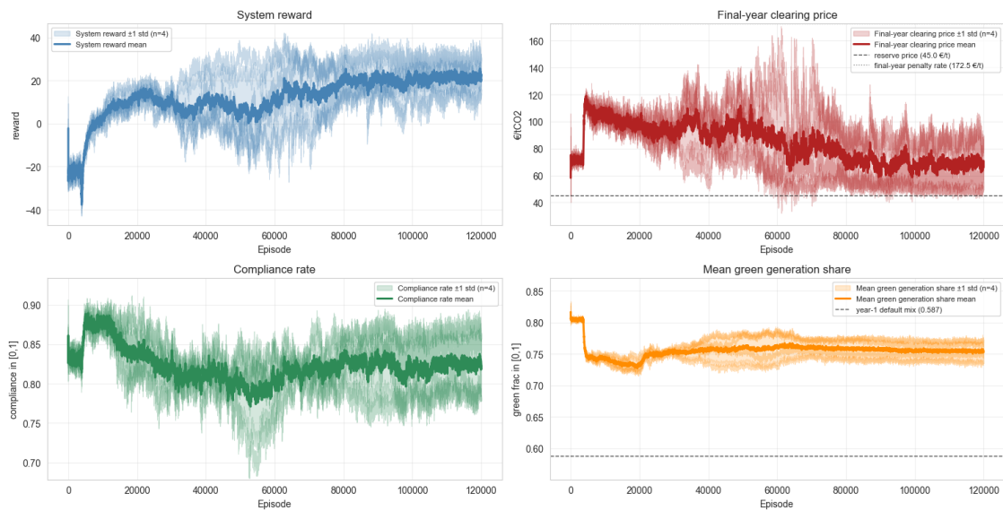
RQ1.5 — Whole-training overview across 4 loaded run(s) (mean ±1 std across runs, ROLL=50)
